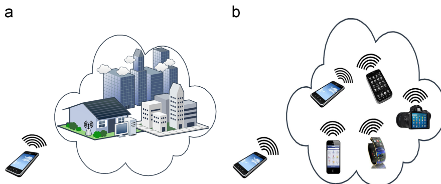
Fig. 3. Cloudlet-based MCC environment. (a) Server-based cloudlet, (b) mobile ad-hoc cloudlet.
