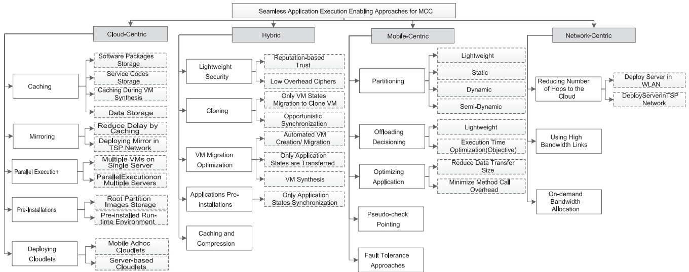
Fig. 5. Taxonomy of seamless execution enabling approaches employed by the CMAEFs for the MCC.
