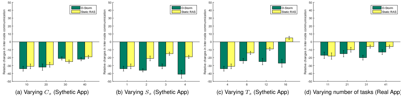
Figure 3. The relative change of the inter-node communication, with the baseline produced by the Default Storm scheduler. We repeated each experiment for 5 times and the result bar also shows the standard deviation of the results. In the legend, static RAS stands for static resource-aware scheduler
