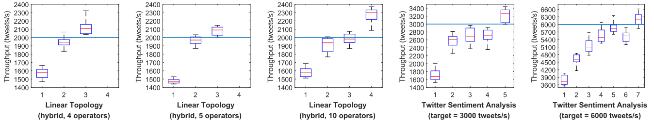
Fig. 11. The monitored throughputs of topologies in the scalability evaluation. Each MAPE iteration corresponds to a plotted box that contains 10 readings of throughputs. P-Deployer finalizes the deployment once the performance target denoted by the horizontal line is reached.
