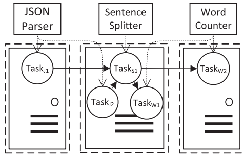
Fig. 3. Partial deployment sketch that shows how to designedly assign the inter-node communication ratio of Task_{s1} to 50 percent. Solid arrows represent data streams while dash arrows denote the “operator-task” containment relationship.
