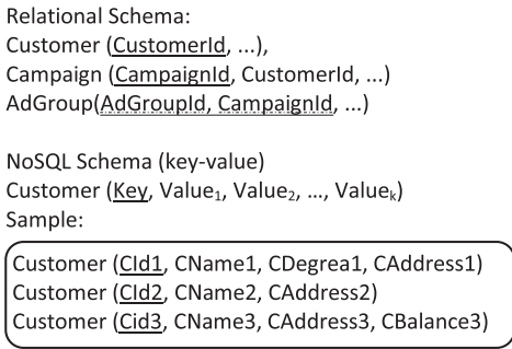
Fig. 2. Relational and NoSQL schemas.
