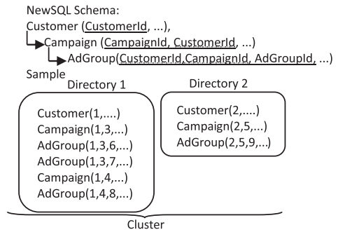
Fig. 3. NewSQL Schema (Shute et al. 2013).
